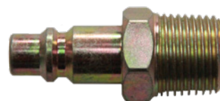
DPM MALE THREAD AIR BRAKE ADAPTER - NON SEALED
