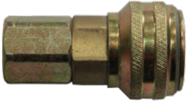
DAF FEMALE THREAD AIR BRAKE COUPLER - SELF SEALED
