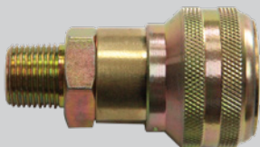
DAM MALE THREAD AIR BRAKE COUPLER - NON SEALED
