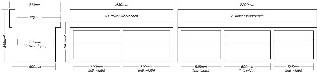
*Drawing heights shown represent the workbench bodies only - excluding the 278mm removable legs.
